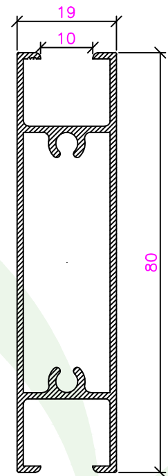
CE-001-61024 Almofada Central
