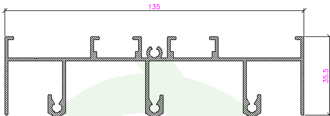
CE-001-90027 Padieira Tri-Rail
