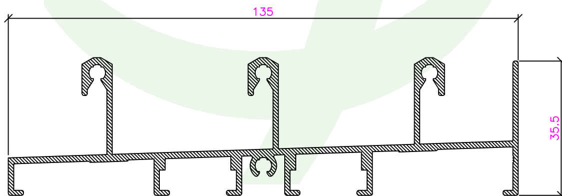
CE-001-90029 Soleira Tri-Rail
